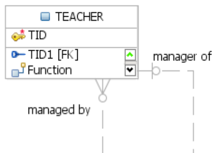
Figure 3.9 – Example of a unary relationship set
