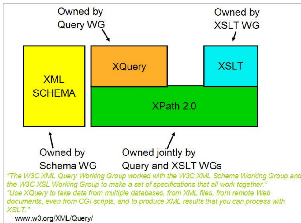
Figure 8.6 - XQuery and related standards
