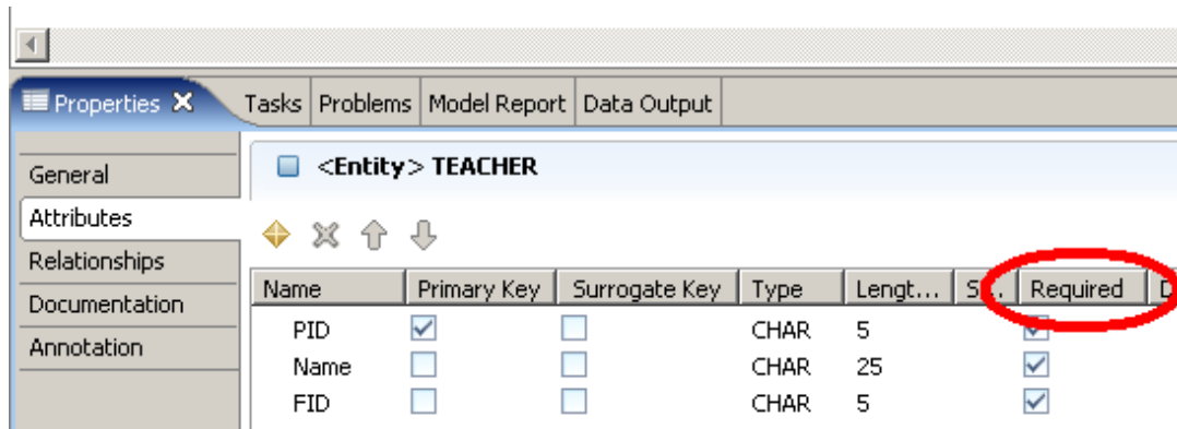
Figure 3.4 - Setting an attribute as mandatory
