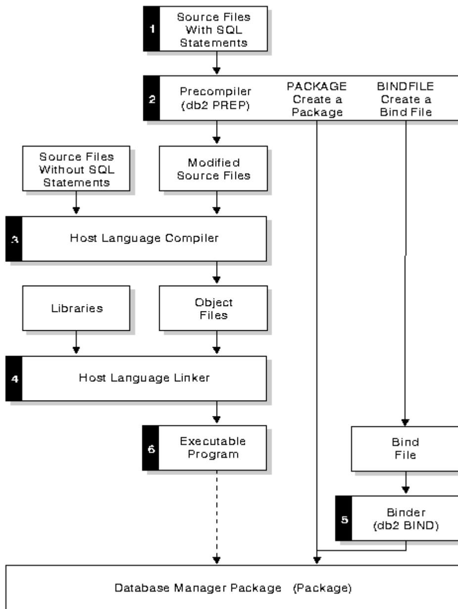
Figure 7.2 -Static SQL compilation and execution process
