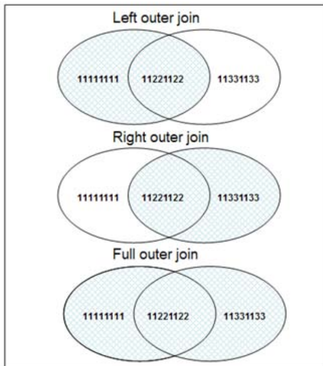
Figure 5.1 - The different outer join types
