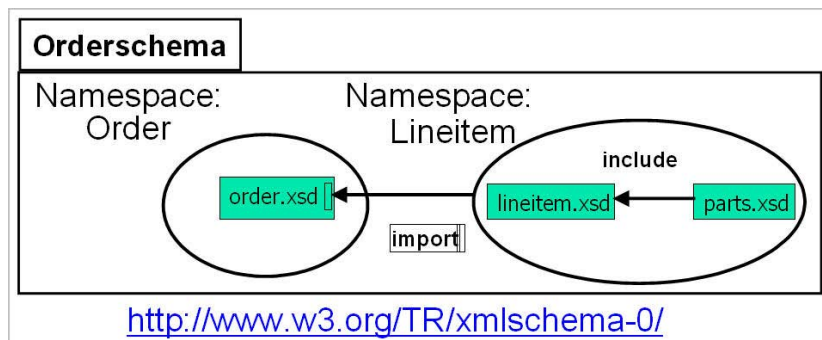
Figure 8.3 - Multiple namespaces in an XML Schema
