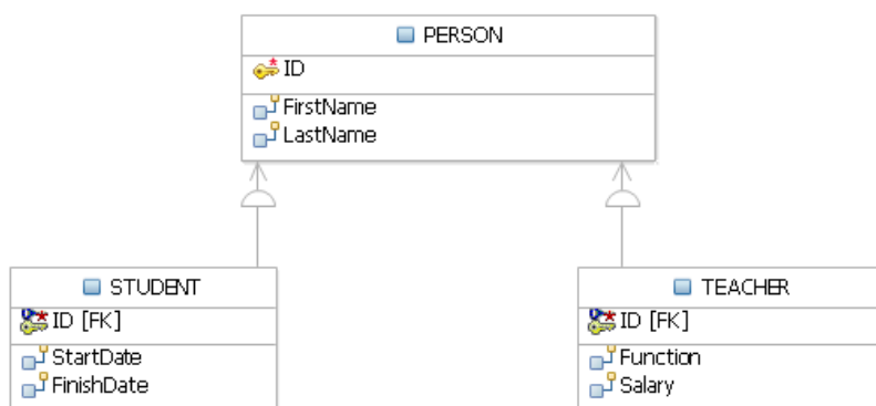
Figure 3.7 - PERSON superset, and its respective STUDENT and TEACHER subsets
