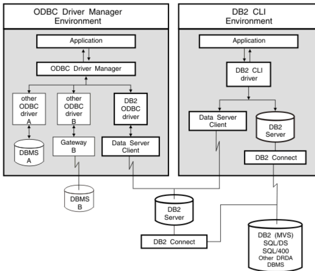
Figure 7.4 - IBM DB2 CLI and ODBC
