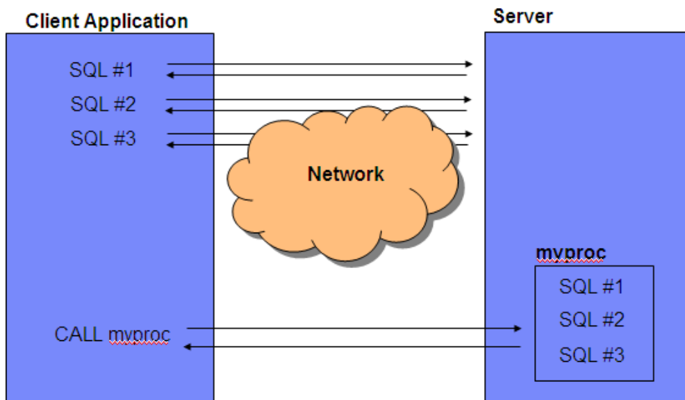
Figure 6.2 – Network traffic reduction with stored procedures
