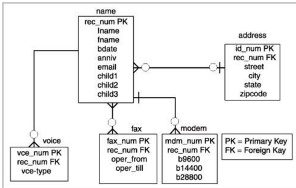
Figure 1.5 - An E-R Diagram for a telephone directory data model
