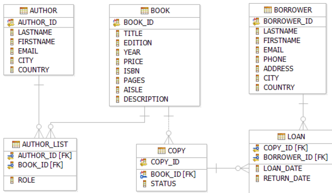
Figure 4.7 – The final logical model
