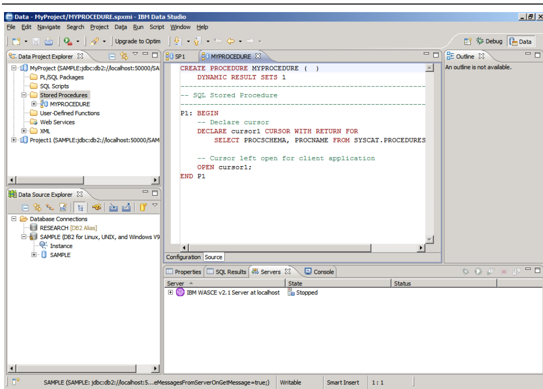
Figure 6.3 – A sample stored procedure
