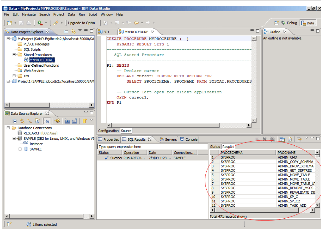
Figure 6.5 – Output after running a stored procedure
