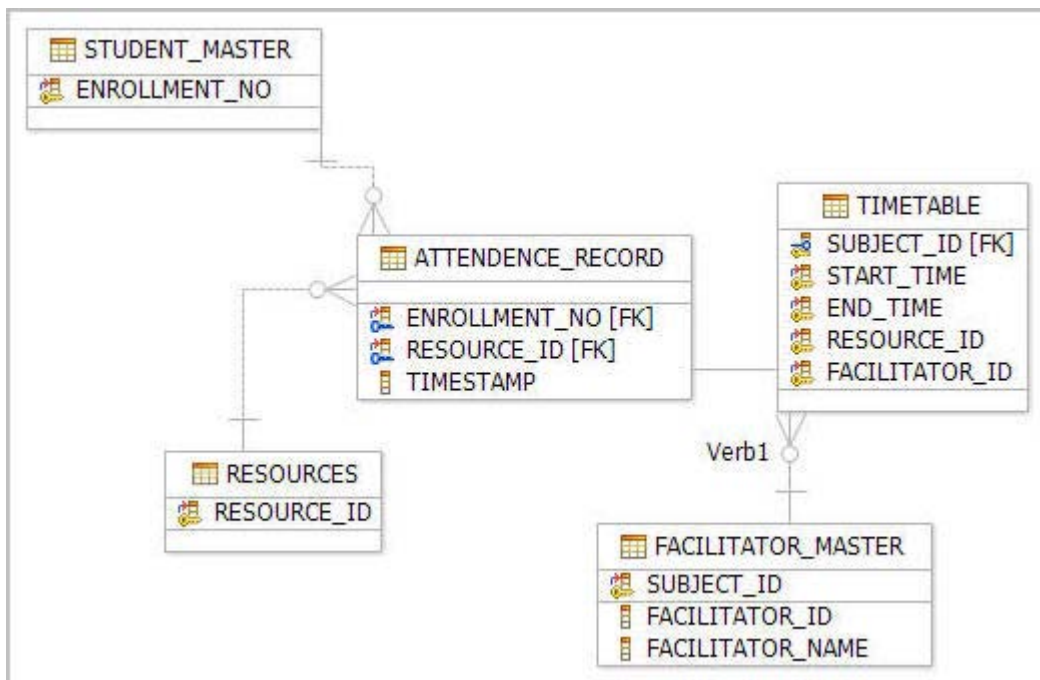
Figure 1.4 - An E-R diagram showing a sample relational model
