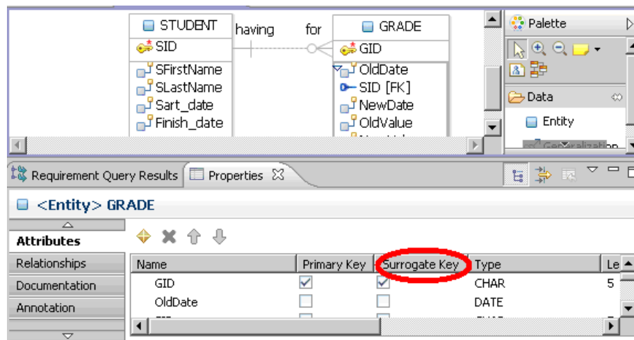
Figure 3.5 - Adding a surrogate key
