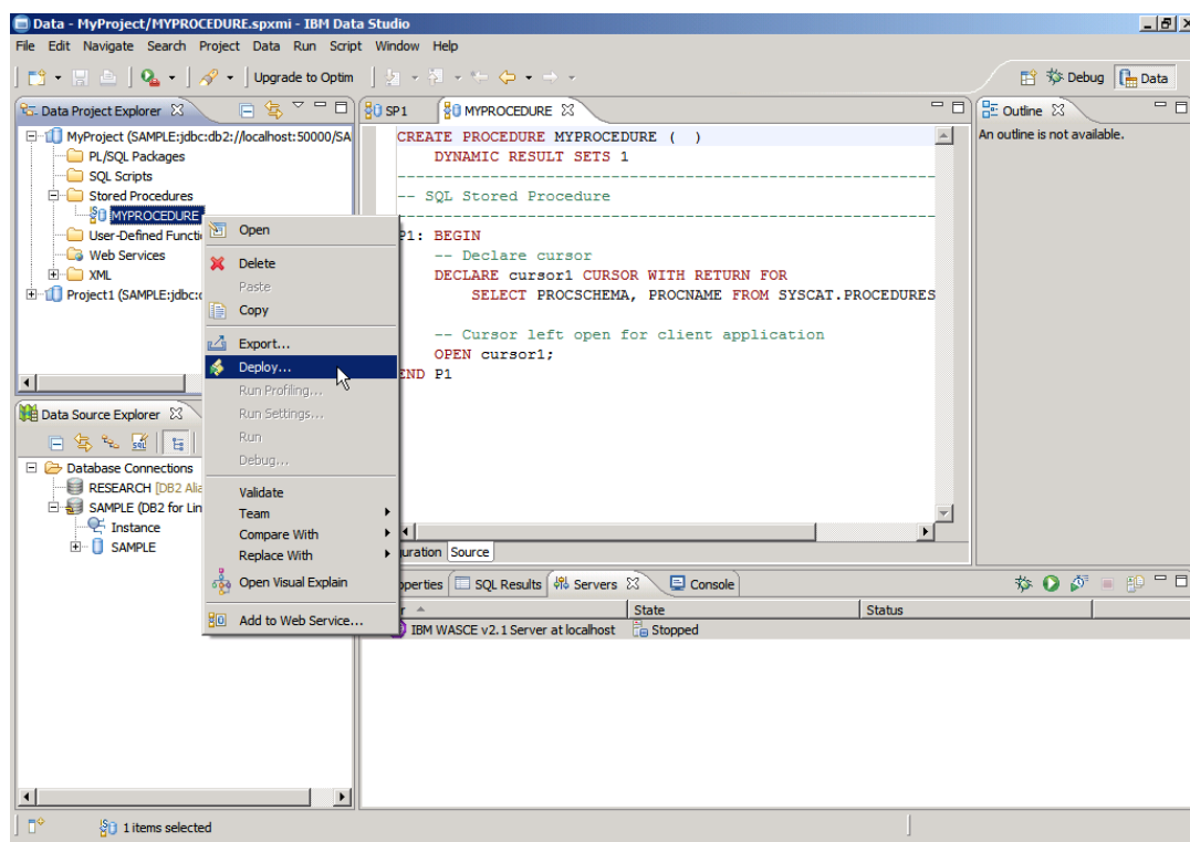
Figure 6.4 – Deploying a stored procedure
