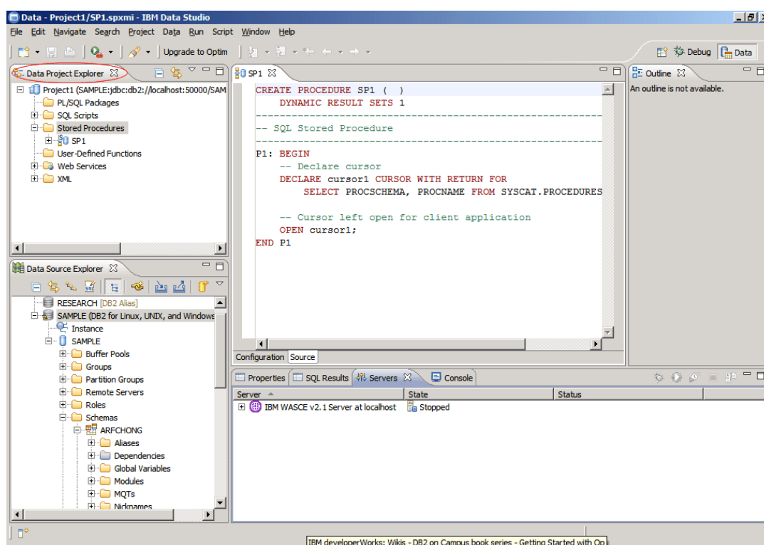
Figure 6.1 – IBM Data Studio 2.2
