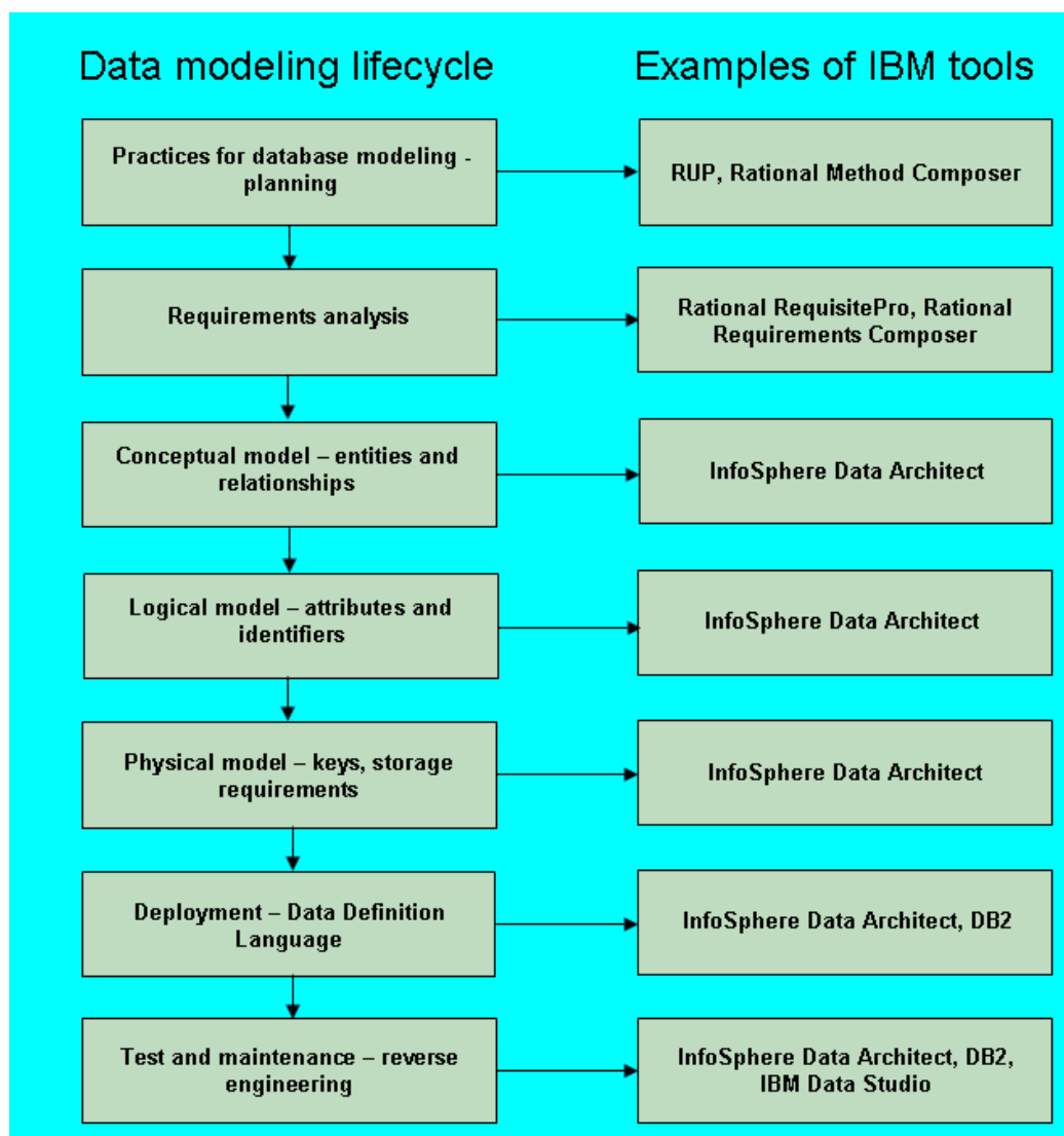
Figure 3.1 - Conceptual, logical and physical modeling within the data modeling lifecycle
