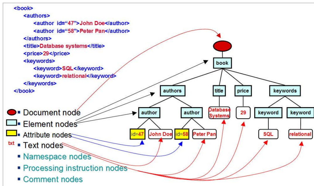
Figure 8.5 - XML Data Model: Node Types
