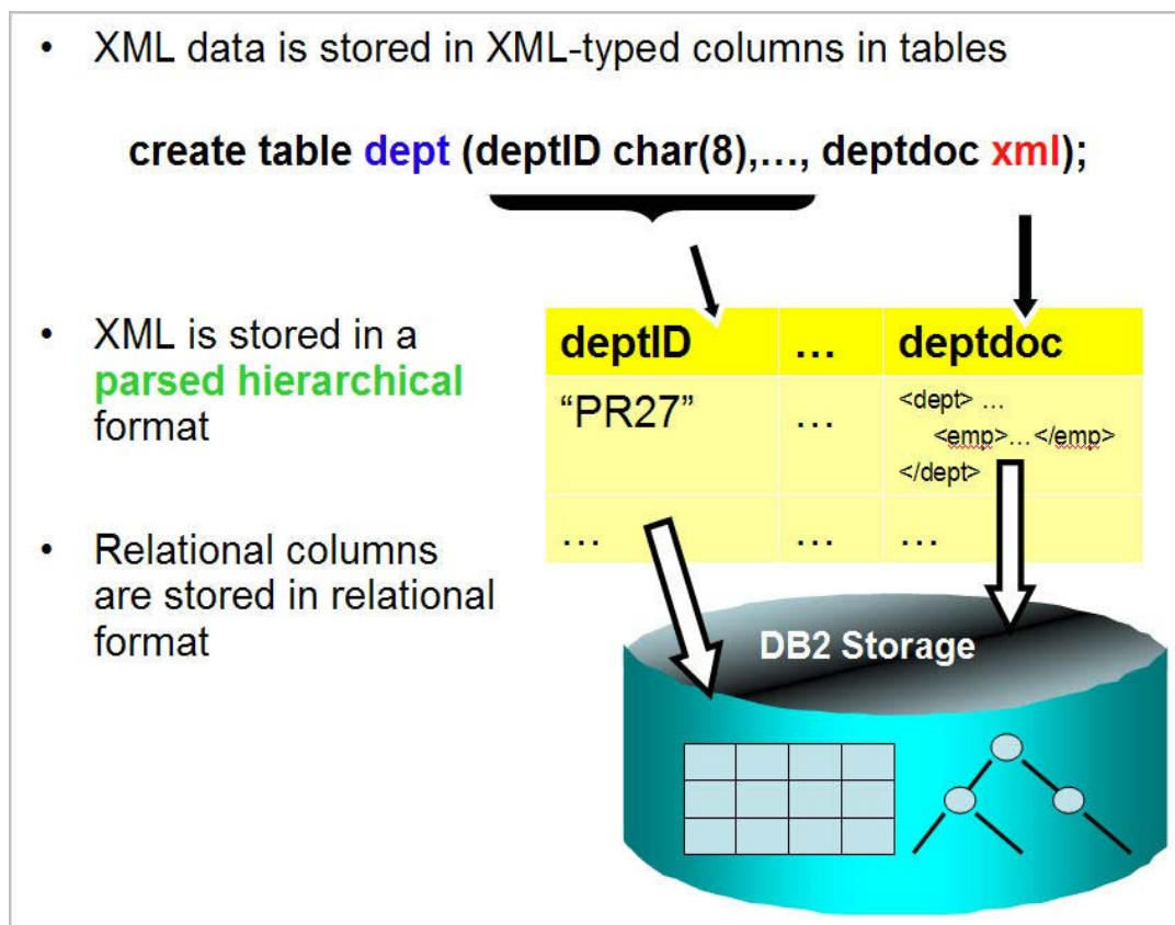
Figure 8.1 - Native XML Storage
