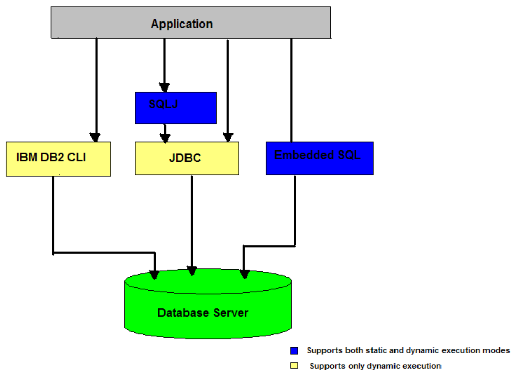
Figure 7.1 - Summary of all the SQL application techniques
